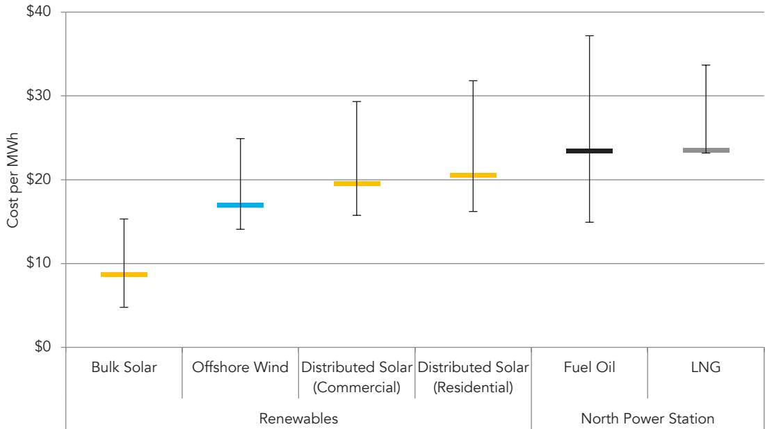
Figure 13 – Levelized energy costs per MWh calculated for this study, in 2017 dollars
