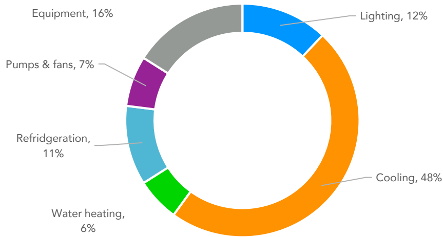
Figure 8- Assumed historical breakdown of hotel energy consumption based on use type
