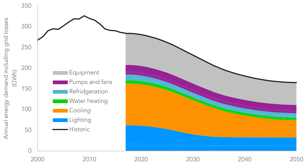
Figure 10 – Projected commercial energy demand with approximate break down by end use
