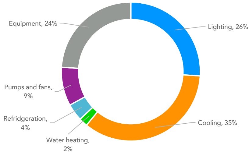
Figure 7 – Assumed historical breakdown of office energy consumption based on use type
