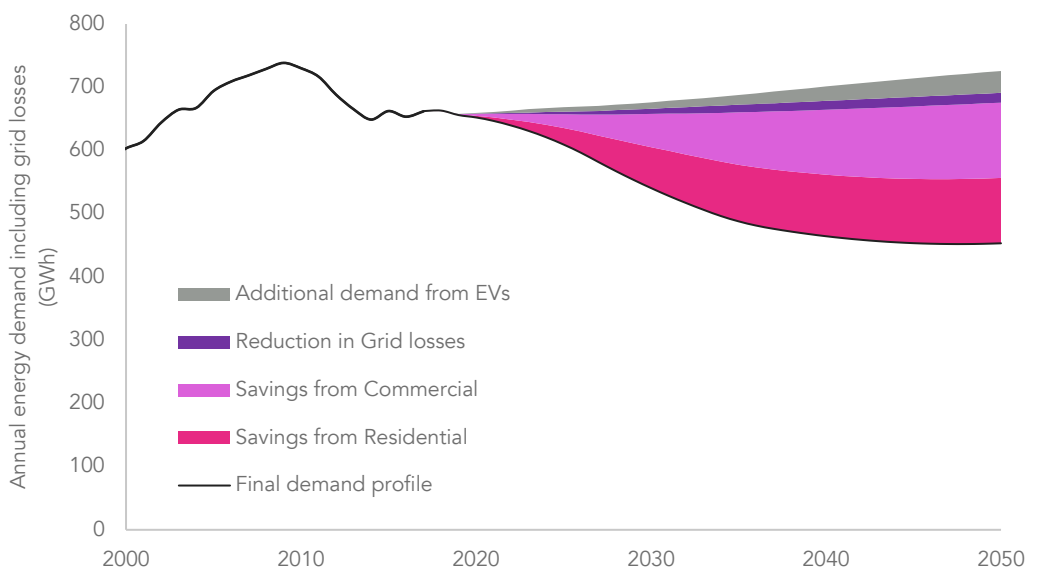
Projected energy demand up to 2050 showing additional demand from electric vehicles, and savings projected from commercial and residential efficiency.
