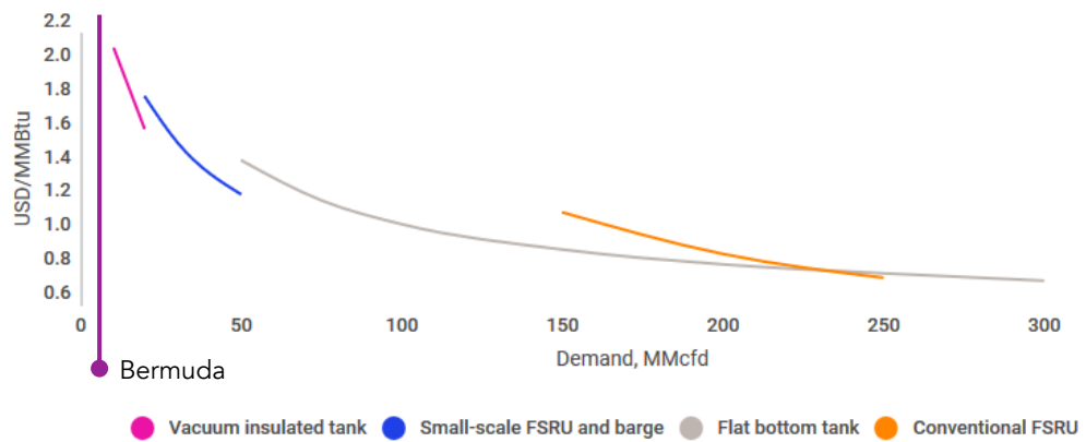
Figure 23 – Regasification cost based on daily demand (©McKinsey 34 )
