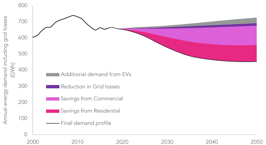
Figure 11 – Projected energy demand up to 2050 showing additional demand from electric vehicles, and savings projected from commercial and residential efficiency.
