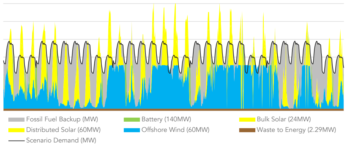
Figure 17 – Hourly dispatch modelling for July in the optimum renewables scenario
