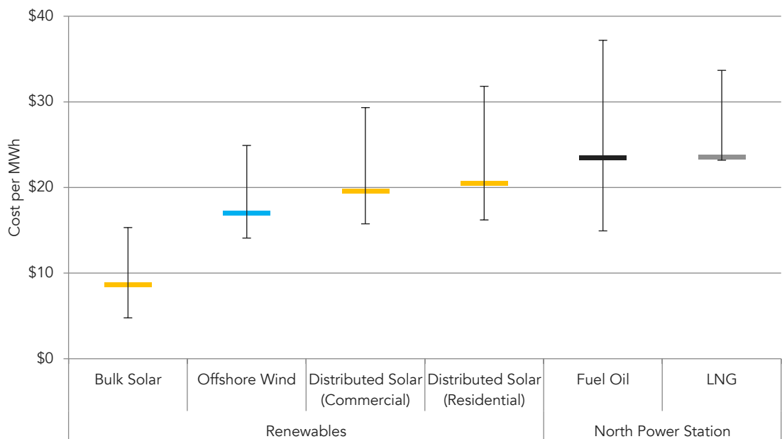
Results of levelized cost of energy calculations. (Coloured bars indicated reference scenarios used in dispatch modelling)
