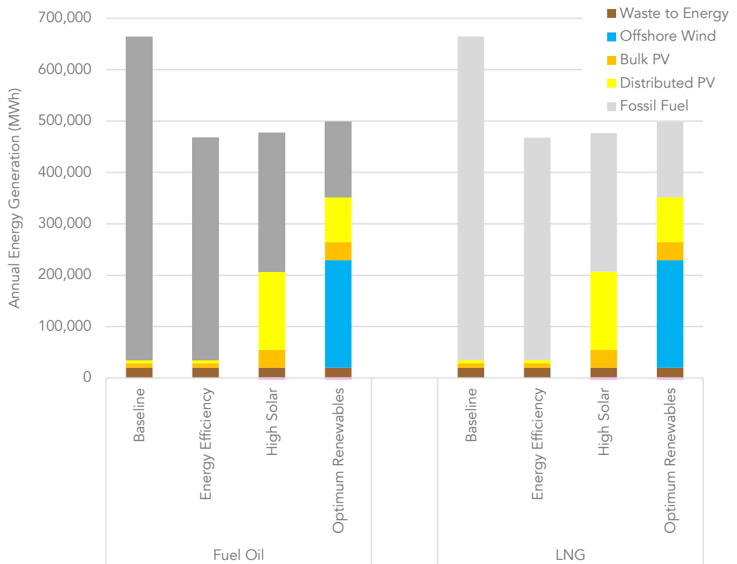
Figure 16 – Annual energy generation from dispatch modelling
