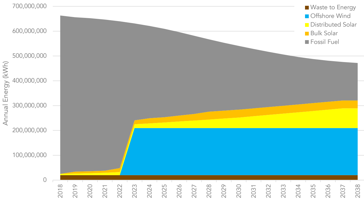
Figure 21 – Bermuda’s changing energy mix in the optimum renewables scenario
